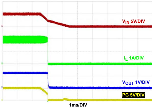
FIGURE 12. SHUTDOWN V_{IN} AT 2A LOAD, f_{SW} = 2\text{MHz} , V_{IN} = 5\text{V} , T_A = +25^\circ\text{C}
