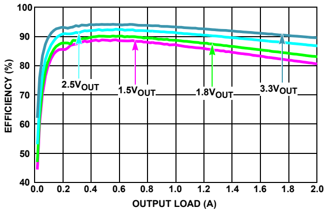
FIGURE 10. EFFICIENCY vs LOAD, f_{SW} = 2\text{MHz} , V_{IN} = 5\text{V} , T_A = +25^\circ\text{C}
