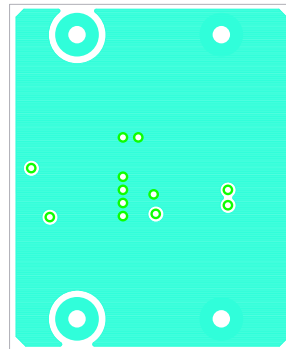
FIGURE 7. LAYER 3
