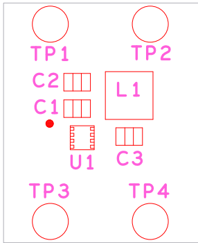
FIGURE 4. SILKSCREEN TOP
