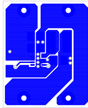
FIGURE 5. LAYER 1
