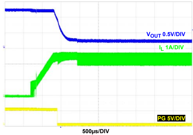
FIGURE 13. OVERCURRENT PROTECTION, f_{SW} = 2\text{MHz} , V_{IN} = 5\text{V} , T_A = +25^\circ\text{C}
