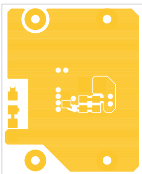
FIGURE 8. LAYER 4
