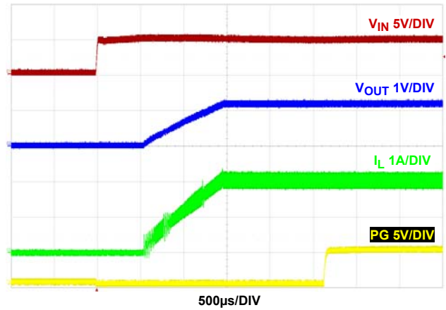
FIGURE 11. START-UP V_{IN} AT 2A LOAD, f_{SW} = 2\text{MHz} , V_{IN} = 5\text{V} , T_A = +25^\circ\text{C}
